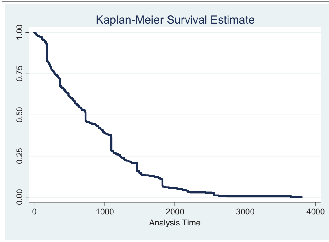
Figure I: Graphical Illustration of Kaplan-Meier Survival Estimate
